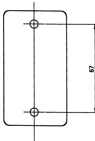
FIXING HOLES
